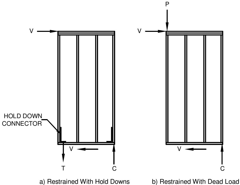
Figure 4: Engineered Shear Wall Restraint Methods
