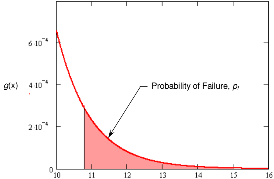
Graph 5: Failure Region of PDF of Shear Wall Load
